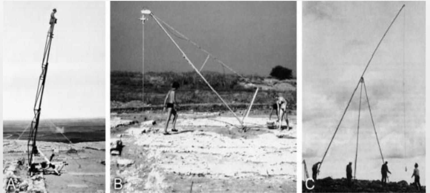
Figure 2. (A) An extendible ladder (Guy, 1932, plate IV). (B) The Holmesboom (Pouter and Kerslake, 1997, figure 6). (C) The phototurret (Nyle, 1964, figure 1).
